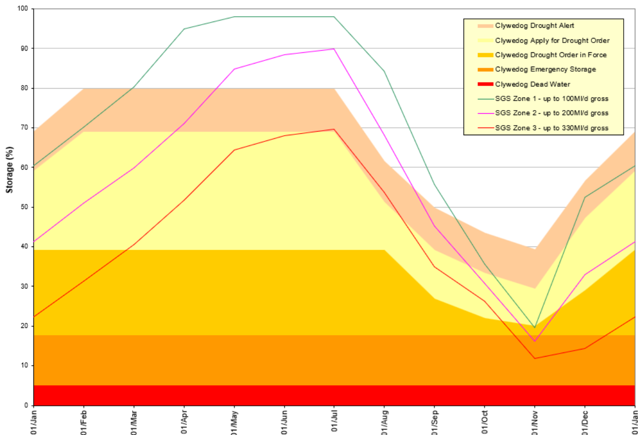
Figure 3. RSDO and SGS Curves - Clywedog Reservoir
