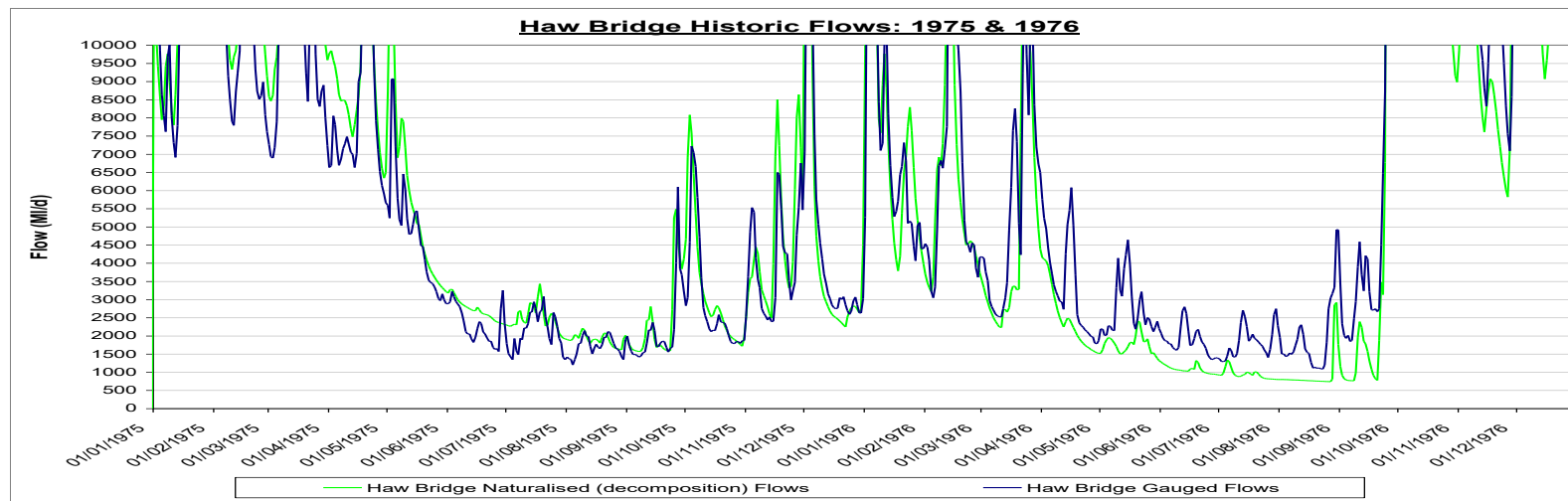
Figure 5. Gauged and naturalised flows at Haw Bridge
