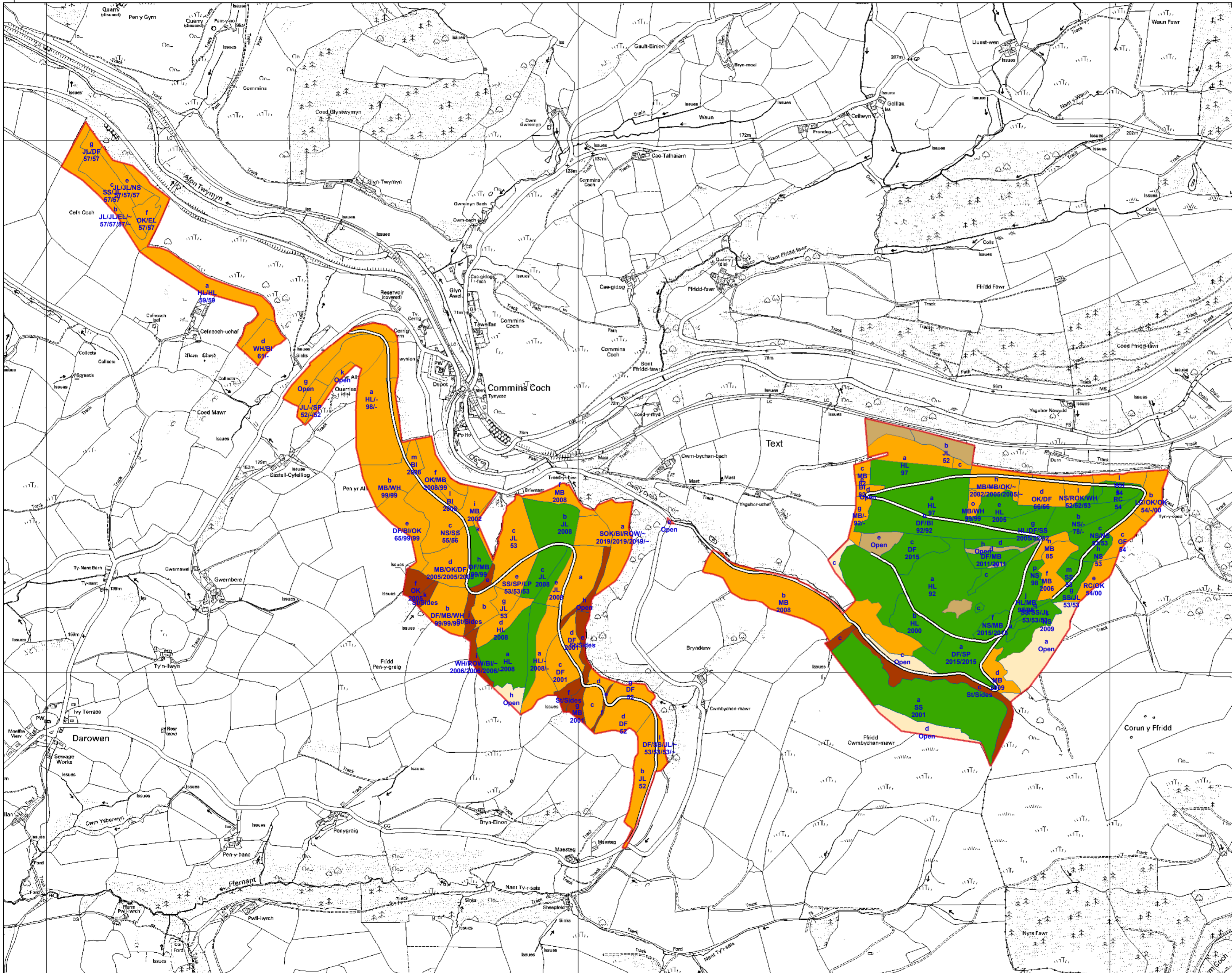
Map 3 Indicative Forest Types
